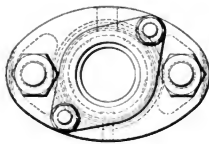
Figs. 2095-2096. Multiangular Packing for 2-in. Valve Stems on Atlantic (4-1-2) Locomotive. P. R. R.
